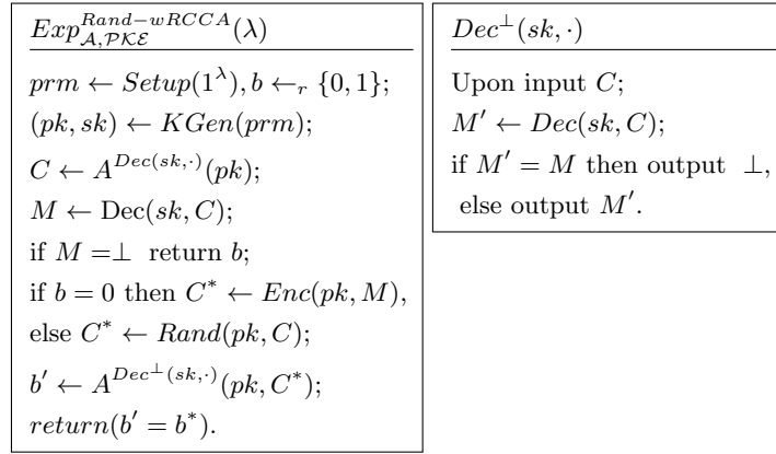
Fig. 2. Weak Re-randomizable RCCA encryption
